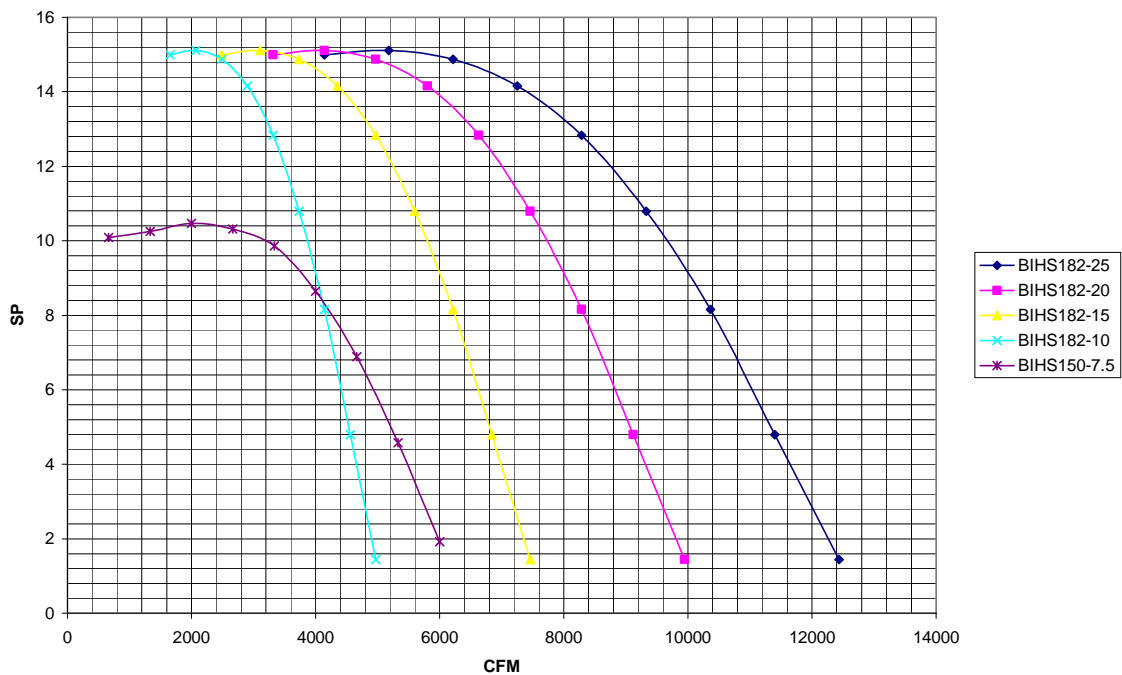
BIHS ARR 4V PERFORMANCE CHART
